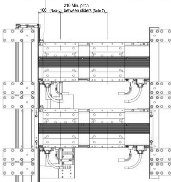
2-slider traverse (Note 6)
