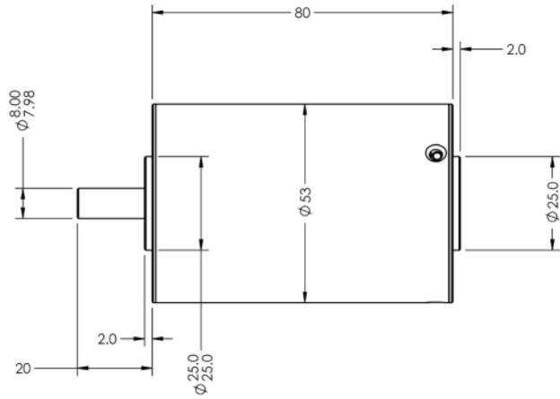
motor alone
