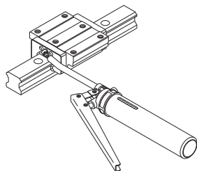
Fig.1 Lubrication using a grease gun
