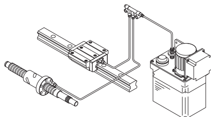
Fig.2 Forced lubrication method
