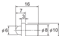
NP8×9 type
