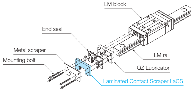
Exterior Drawing
