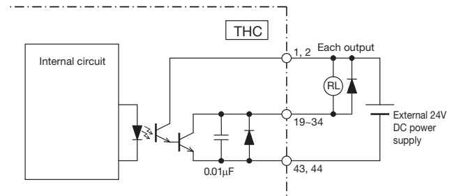
Output circuit
