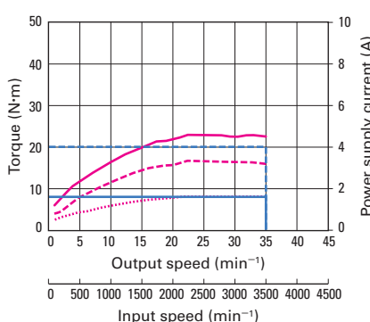
⑤ Motor model number PBM603FHMK30-M
