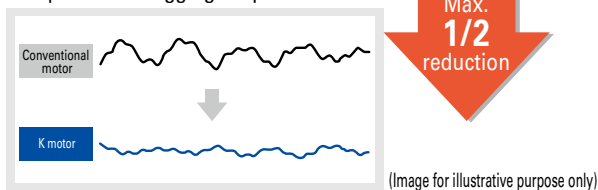
Comparison of cogging torque waveforms
