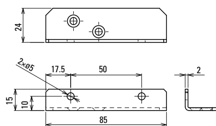
Lower bracket
