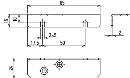
Lower bracket
