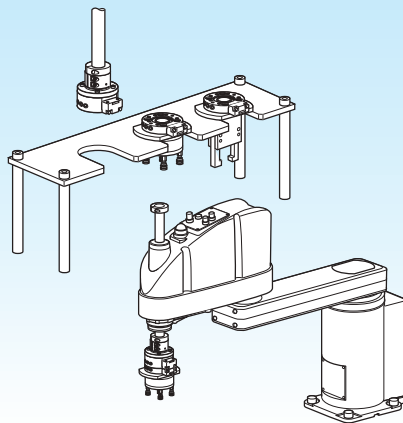
② Attach to auto hand changer
