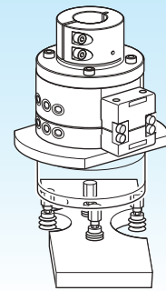
③ Fall prevention check valve (option) to prevent falling of workpieces due to suction failure
