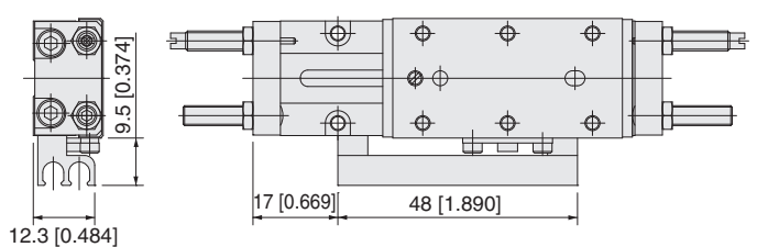
When magnet and sensor rail installed (Piping direction-L)
