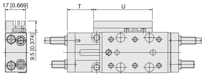
When magnet and sensor rail installed (Piping direction-R)
