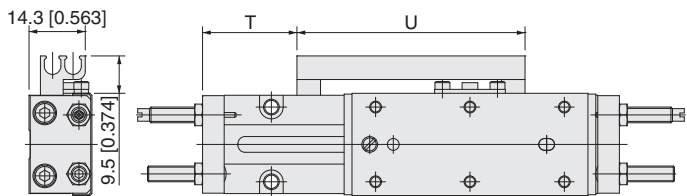
When magnet and sensor rail installed (Piping direction-R)
