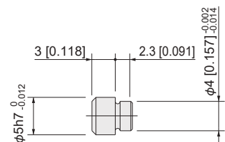
Locating pin hole:-P (P-MGA2)
