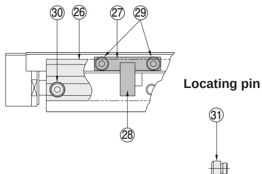
MGAES□ (with magnet and sensor rail)
