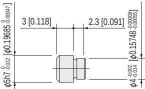
Locating pin: -P (P-MGA2)
