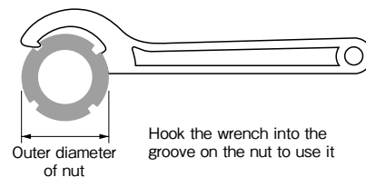
Hook wrench
