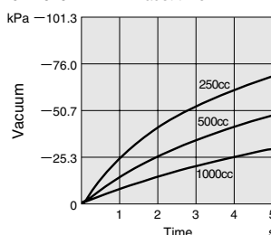
GAV010LE1-11 Exhaust time
