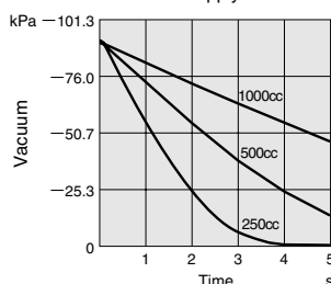
GAV010HE1-11 Air supply time
