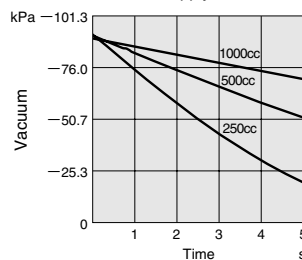
GAV010LE1-11 Air supply time
