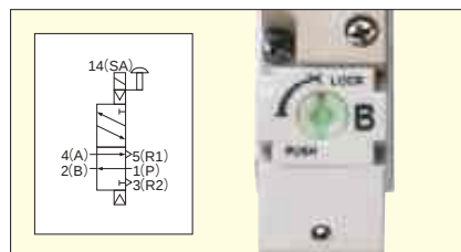
Single solenoid position
