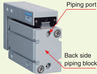
Piping port
