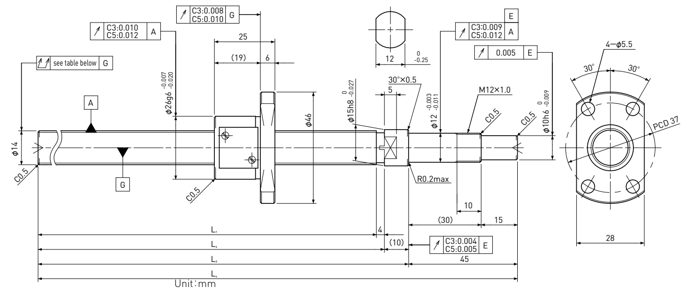
Supported-side end-journal profile
