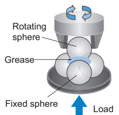
Testing apparatus
