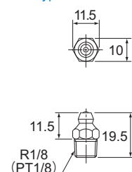
A-PT1/8 type
