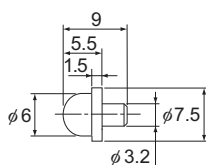
NP3.2×3.5 type
