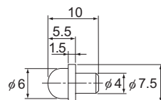
PB1021B type
