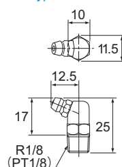
B-PT1/8 type
