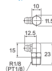
C-PT1/8 type
