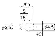
PB107 type
