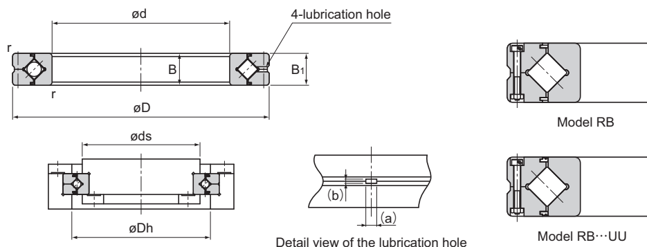
Detail view of the lubrication hole
