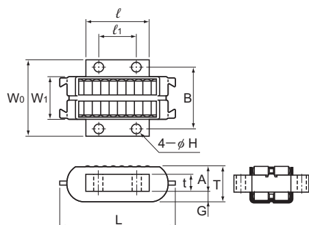
Model LR
