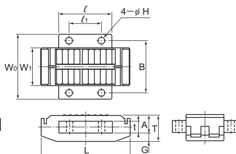
Model LR-Z
