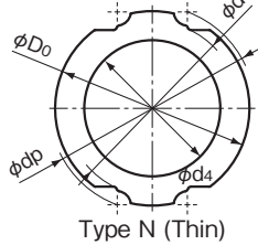
Cross-Sectional Shapes of Spline Shafts
