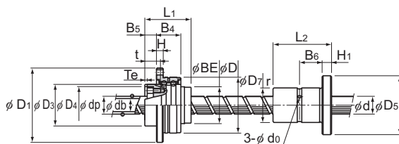
Ball screw unit
