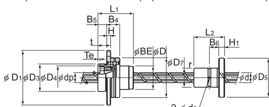
Ball screw unit
