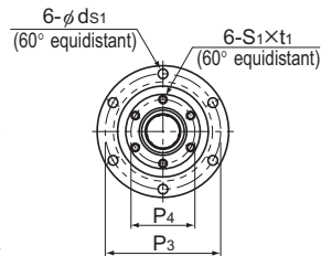
Ball spline
