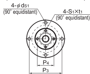
Ball spline
