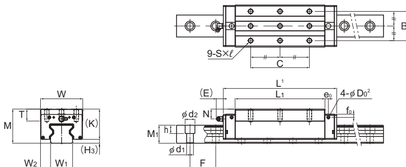
Models SRG35 and 45 SLR
