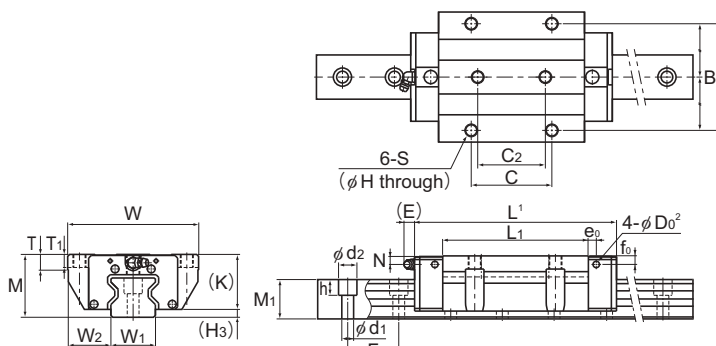
Models SRG25X and 30X C/LC
