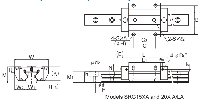
Models SRG15XA and 20X A/LA
