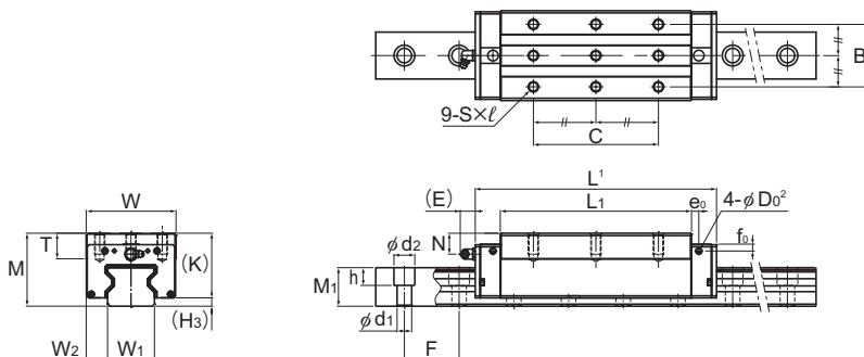
Models SRG55SLR and 65SLV
