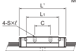
Models RSX7 to 12WM/WMN
