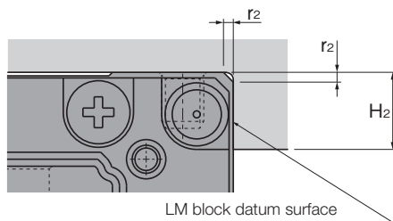
LM block
