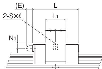
Model AHR15S
