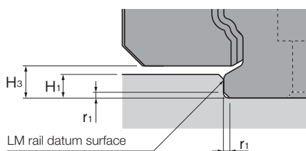
LM rail
