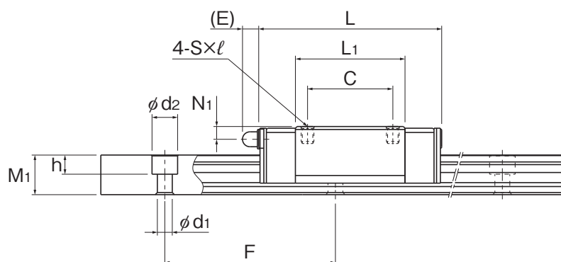
Models AHR15M/N
